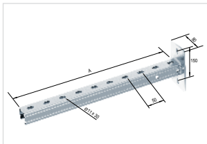
CE SR41 Soporte rail 41x41
