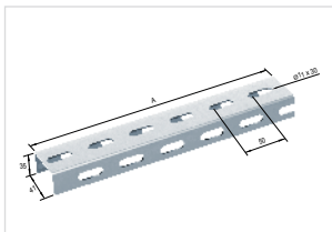
CE RU4135 Rail "U" 41x35
