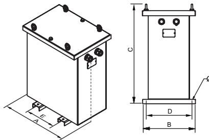
TKZ IP65
